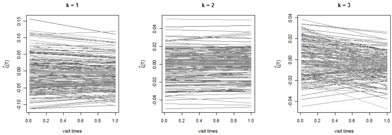
Figure 3. Estimated time-varying coefficients \hat{\xi}_{ik}(T) for k = 1, 2 and 3 using REM
