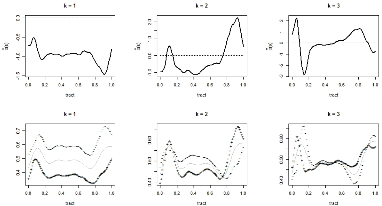
Figure 2. Top: First three eigenfunctions of the estimated marginal covariance; Bottom: estimated mean function \hat{\mu}_0(s) (gray line) \pm 2\sqrt{\lambda_k}\hat{\phi}_k(s) (+ and - signs, respectively)
